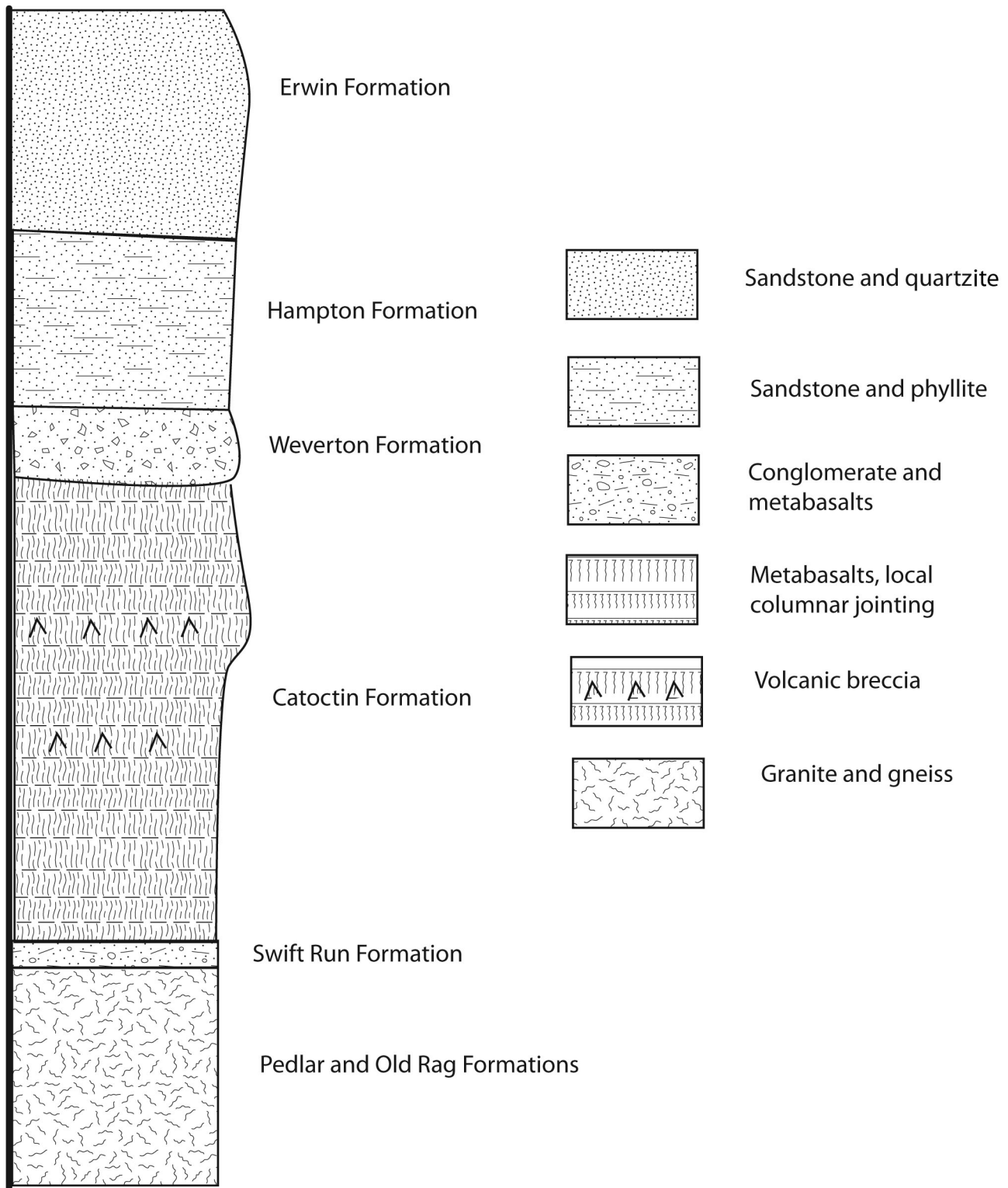
Simplified Stratigraphic Column for Shenandoah National Park
